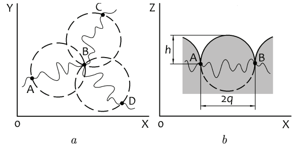
Fig. 3. Polymer coils at the gel surface: the view from above ( a ), the surface cross-section by a plane parallel to the Z axis ( b )
