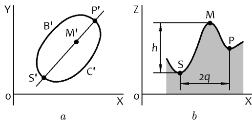
Fig. 2. Protrusion on the gel surface: the view from above ( a ), the protrusion cross-section by a plane parallel to the Z axis ( b )
