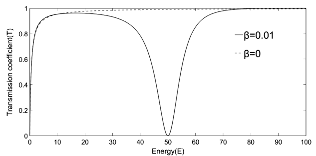
Fig. 2. Transmission coefficient for \beta = 0.01 (solid line) and \beta = 0 (dotted line) [Eq. (28)]
