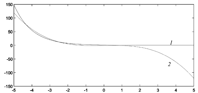
Fig. 3. Graphs of Eq. (39) taking e^{-z}(1) and z - z^3 - 1(2)
