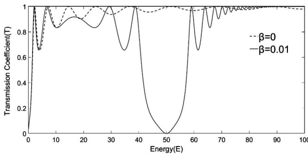
Fig. 5. Transmission coefficient for \beta = 0.01 (solid line) GUP case and \beta = 0 (dotted line) non-GUP case [Eq. (45)]
