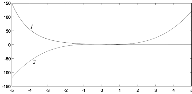
Fig. 4. Graphs of Eq. (43) taking e^{-z} (1) and 1 - z + z^3 (2)
