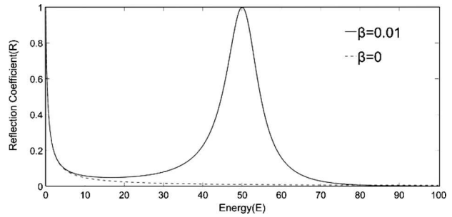
Fig. 1. Reflection coefficient for \beta = 0.01 (solid line) and \beta = 0 (dotted line) [Eq. (27)]
