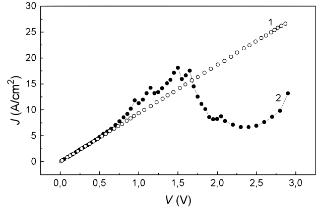
Fig. 1. Typical current-voltage characteristics (CVCs) of \text{In}_2\text{Se}_3 samples with a thickness of 600 \mu\text{m} at the temperature T = 289 \text{ K} : linear (curve 1), Z - and N -shaped (curve 2)
