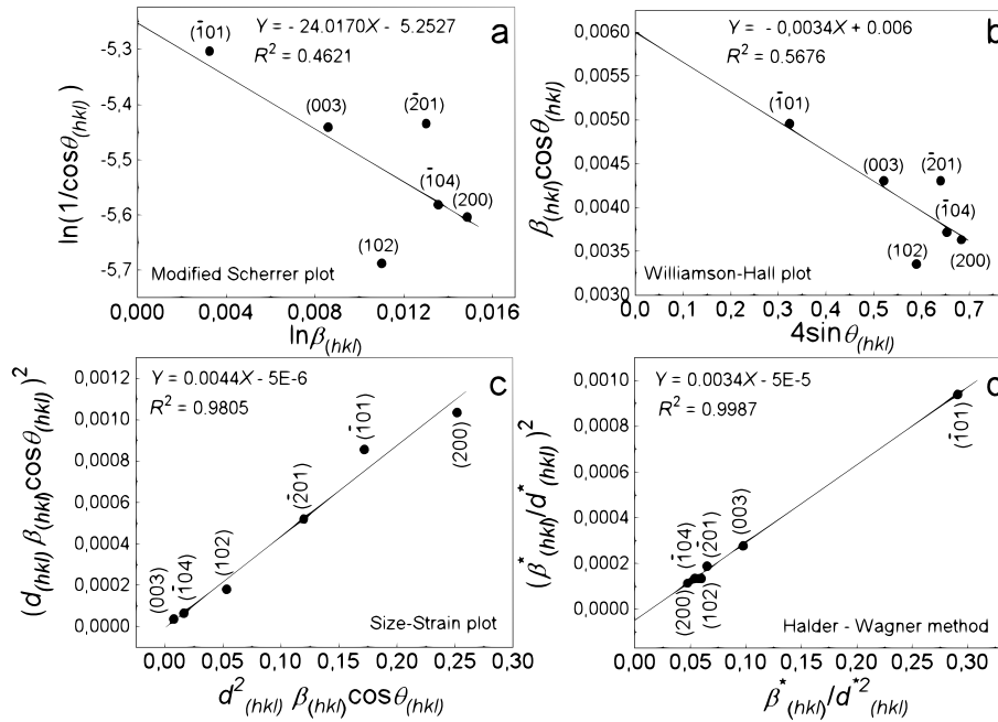
Fig. 3. Modified Scherrer (a), Williamson–Hall (b), SSP (c), and Halder–Wagner (d) dependences plotted to characterize \text{In}_6\text{Se}_7 nanocrystallites in the layered \alpha\text{-In}_2\text{Se}_3 matrix. R^2 is the reliability of approximation of experimental data (symbols) by the corresponding dependence (lines)
