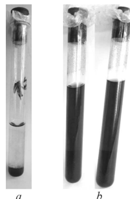
Fig. 9. Express analysis of the content of the soluble component of soot fractions C_{60} and C_{70} : does not confirm the presence of fullerenes C_{60} and C_{70} in the first three samples (Table 3, items 1, 2, and 3) ( a ); confirms the presence of fullerenes C_{60} and C_{70} in the last two samples (Table 3, items 4 and 5) ( b )
