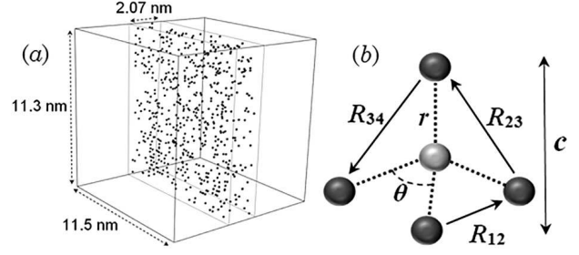
Fig. 1. Schematic diagram of a 2.07-nm-thick quantum well for which the calculations were performed (points demonstrate one of the random distributions of indium atoms in the well) (a). The arrangement of the nearest neighbor atoms in the hexagonal crystal structure and the vectors defining the geometry of this arrangement (b)
