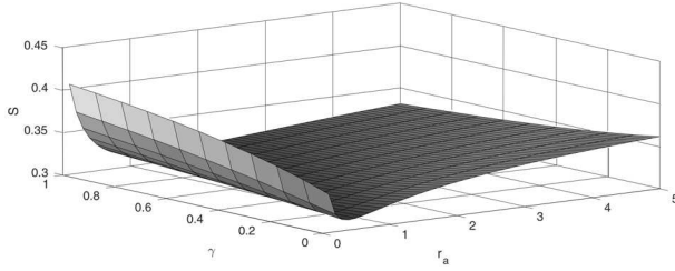
Fig. 5. Plot of the quadrature squeezing at the steady state, [Eq. (168)] versus r_a and \gamma for \kappa = 0.8 , \gamma_c = 0.4 , M_0 = 0.59 , and N_0 = 0.27
