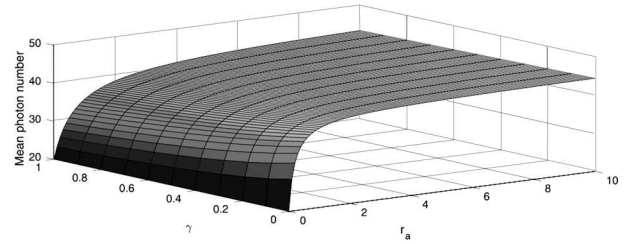
Fig. 3. Plots of the mean photon number for the two-mode cavity light at the steady state [Eq. (135)] for \kappa = 0.8 , \gamma_c = 0.4 , N_0 = 0.2 , and N = 50 vs \gamma and r_a
