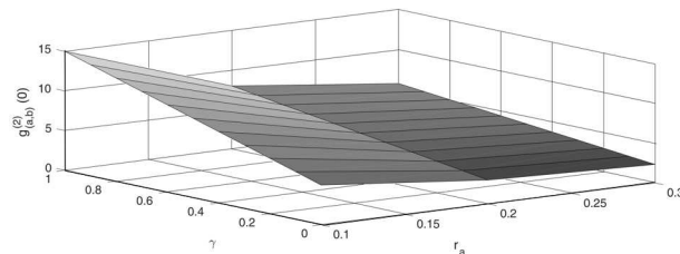
Fig. 9. Plots of g_{(a,b)}^{(2)}(0) of the two-mode cavity light versus r_a and \gamma for \gamma_c = 0.4
