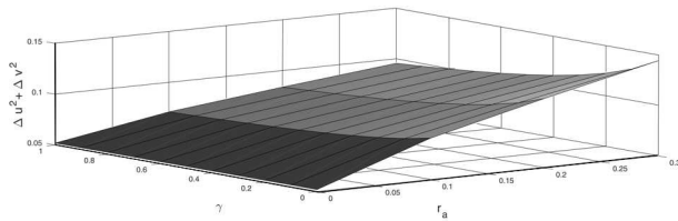
Fig. 7. Plots of \Delta u^2 + \Delta v^2 of the two-mode cavity light versus r_a and \gamma for \gamma_c = 0.4
