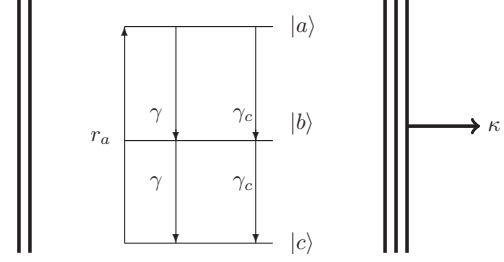
Fig. 1. Schematic representation of a three-level laser coupled to a two-mode squeezed vacuum reservoir
