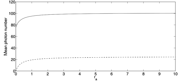
Fig. 2. Plots of the mean photon number for the two-mode cavity light at the steady state [Eq. (135)] for \kappa = 0.8 , \gamma_c = 0.4 , \gamma = 0.2 , N_0 = 0.2 (solid curve), N_0 = 0 (dashed curve), and N = 50
