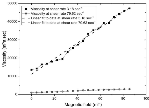
Fig. 6. The measured viscosity as a function of the magnetic field at a low shear rate ( 3.18 \text{ sec}^{-1} ), and at a higher shear rate ( 79.62 \text{ sec}^{-1} )
