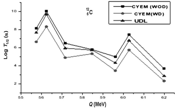
Fig. 2. Plot for \text{Log} T_{1/2} (s) vs. Q (MeV) of ^{12}_6\text{C} cluster emitted from various parent nuclei
