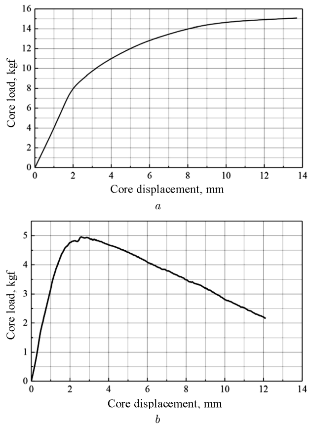
Fig. 3. Force characteristics of magnetic springs: basic model ( a ) and spring with the magnetic conductor instead of the outer permanent magnet ( b )
