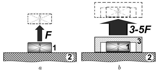
Fig. 2. Schematic diagram of using a magnetic conductor to shift the operating point of the permanent magnet along the demagnetization curve: the permanent magnet is on a ferromagnetic plane ( a ); the same permanent magnet is additionally covered with a magnetic conductor ( b ): permanent magnet (1), ferromagnetic plane (2), magnetic conductor (3)
