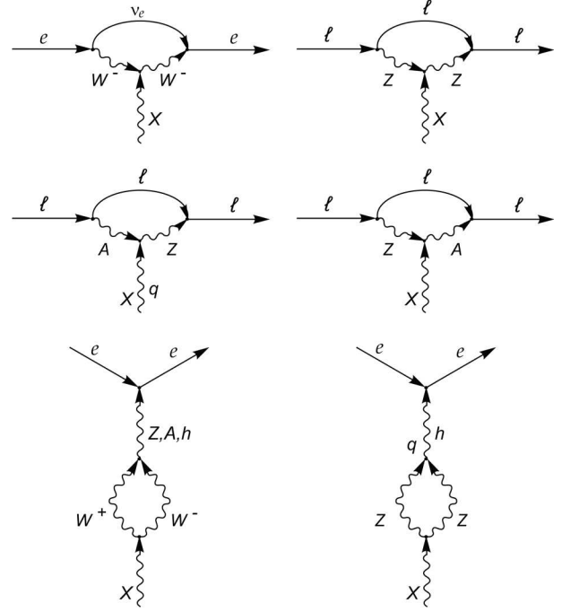
Fig. 3. Diagrams of the CS boson's decay into leptons in the unitary gauge. The interaction depends on c_w , c_\gamma and c_Z couplings
