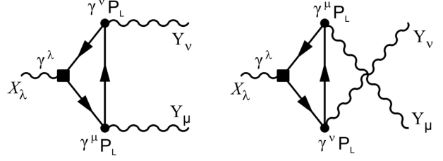
Fig. 1. Diagrams generating the Chern–Simons interaction. Heavy fermions, beyond the Standard Model, run in loop triangular diagrams
