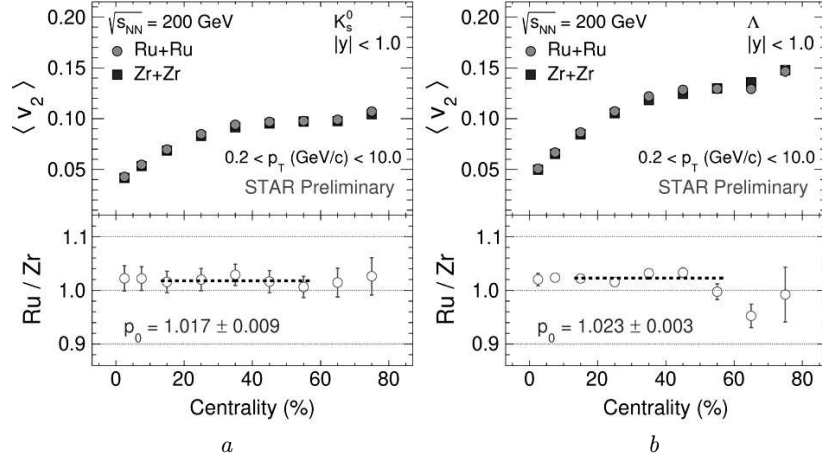
Fig. 8. Integrated elliptic flow ( \langle v_2 \rangle ) as a function centrality (%) for K_s^0 (a) and \Lambda (b) at mid-rapidity ( |y| < 1.0 ) in Ru + Ru and Zr + Zr collisions at \sqrt{s_{NN}} = 200 GeV from the STAR experiment at RHIC. The bottom panels show ratio of \langle v_2 \rangle between Ru and Zr, fitted with a constant polynomial function
