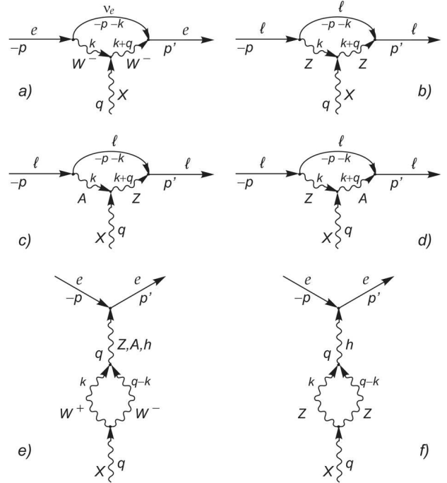
Fig. 1. Diagrams of the CS boson's decay into leptons in the unitary gauge
