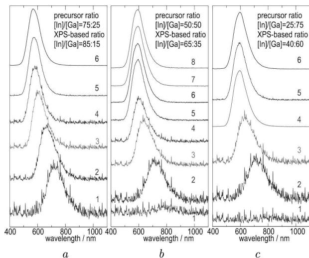
Fig. 3. PL spectra of series of size-fractionated non-stoichiometric GSH-capped Ag-(In,Ga)-S QD solutions prepared with [Ag]:[In]:[S] precursor molar ratio of 1:4:5 and three different [In]:[Ga] precursor molar ratios in the reaction mixture: 75:25 (a), 50:50 (b), and 25:75 (c). The corresponding XPS-estimated [In]:[Ga] ratios in the QDs are indicated in the figure. Size-selected fraction numbers are shown at each curve
