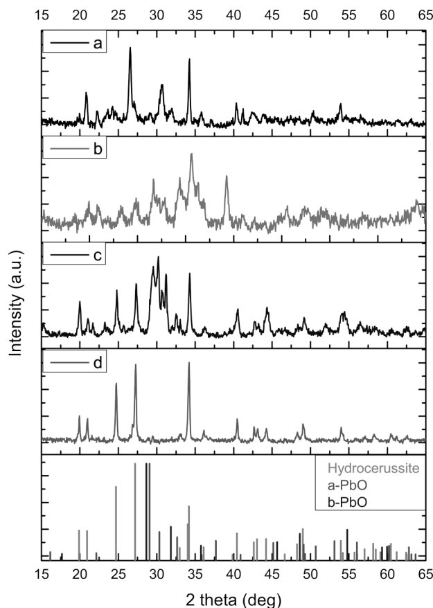
Fig. 1. X-ray diffractograms of specimens and (the bottom panel) X-ray standards of Hydrocerussite, \alpha -PbO, and \beta -PbO. Synthesis parameters: NaCl electrolyte, the synthesis temperature t = 24^\circ\text{C} ( a ); NaCl electrolyte, t = 60^\circ\text{C} ( b ); NaCl electrolyte, t = 98^\circ\text{C} ( c ); Na_2CO_3 \times 10H_2O electrolyte, t = 20^\circ\text{C} ( d )
