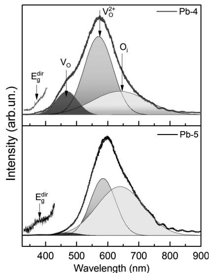
Fig. 2. Micro-PL spectra of PbO powders and the approximation of PL band by Gaussian contours; \lambda_{exc} = 325.0 nm, T = 300 K
