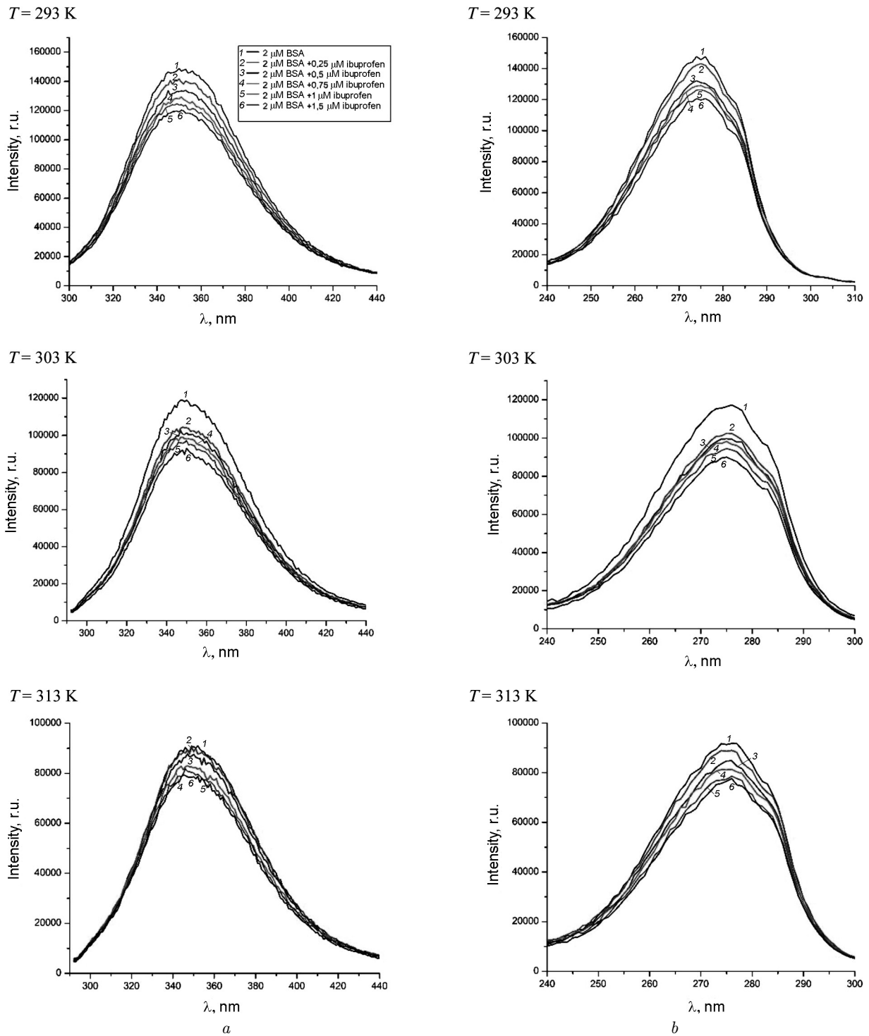
Fig. 2. Emission ( \lambda_{ex} = 353 nm) (a) and excitation ( \lambda_{em} = 275 nm) fluorescence spectra of the aqueous solutions of BSA and ibuprofen at various temperatures (b)
