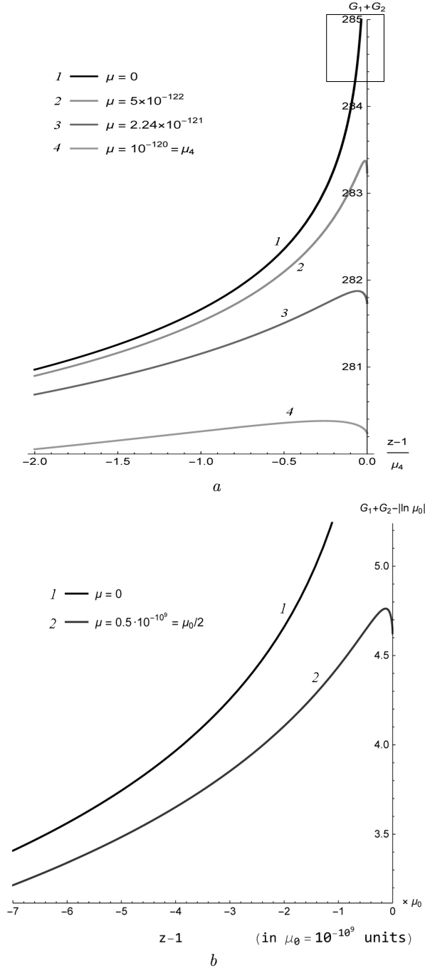
Fig. 3. Dependence of G_1(\mu; z) + G_2(\mu; z) on \delta z \equiv z - 1 measured in the units of largest value \mu_4 , close to z = 1 for \mu \sim 10^{-120} (a). Dependence of G_1(\mu; z) + G_2(\mu; z) on \delta z , shifted by |\ln(\mu_0)| \approx 2.30 \times 10^9 , for the extremely small \mu -scale given by \mu_0 = 10^{-109} , however, with focus on the extremum position (b). This figure roughly corresponds to the box in the up panel
