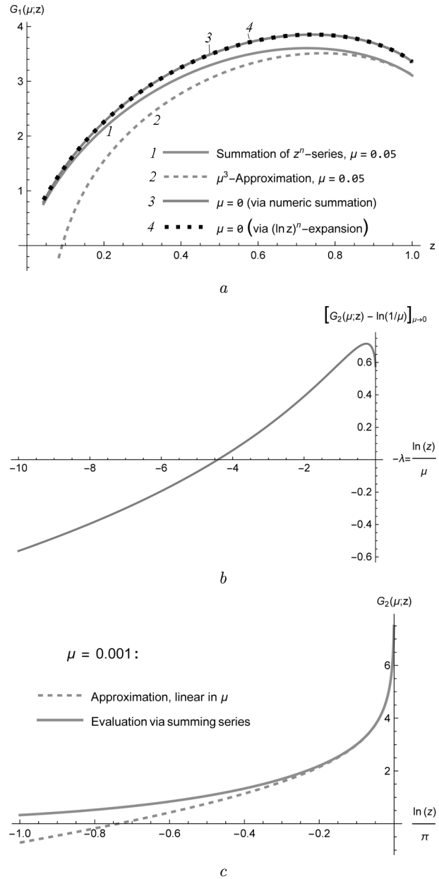
Fig. 1. Dependence of G_1 on z ( a ) and the difference G_2 - \ln \frac{1}{\mu} on -\lambda = \frac{\ln(z)}{\mu} ( b ). The bottom plots show a discrepancy between the approximation and numerical evaluation for G_2 . Pane ( a ): solid curves 1 and 3 show the behaviour of numerically evaluated G_1 basing on the summation of defining z^n -series, resp. for \mu = 0.05 and \mu = 0 ; dashed 2 and dotted 4 curves are obtained via \mu^3 -approximation (50) and (\ln z)^n expansion (54), resp. for \mu = 0.05 and \mu = 0 . Pane ( c ): dashed curve corresponds to linear-in- \mu approximation, see (59) and footnote 1, whilst solid one is evaluated via summing series (for both cases \mu = 0.001 )
