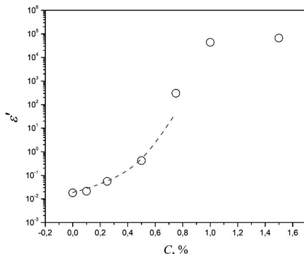
Fig. 2. Concentration dependence of dielectric permittivity for systems based on PLA and CNTs at a frequency of 1 kHz. Dashed curve corresponds to percolation model (1)
