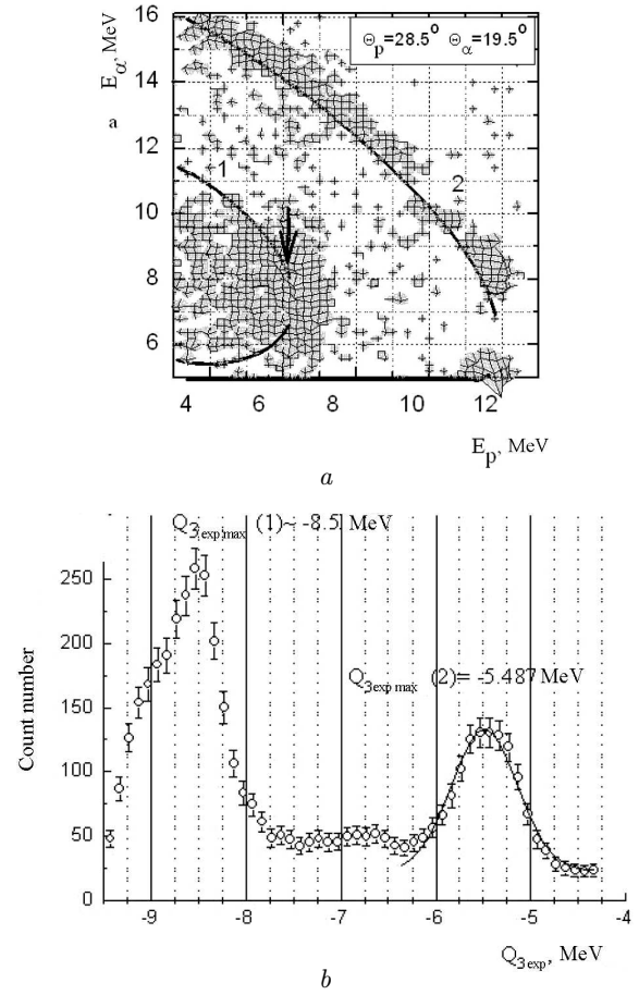
Fig. 1. Two-dimensional p\text{-}\alpha coincidence spectrum (a); the corresponding energy-balance, Q_{3\text{exp}} , spectrum (b)
