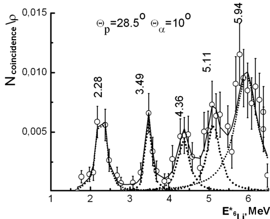
Fig. 2. Projection of the upper branch of the p - \alpha coincidence matrix. The numbers indicate the fitted excitation energies of the first five excited states of the {}^6\text{Li} nucleus. The corresponding individual contributions of excited levels and their sum are shown by the dotted and solid curves
