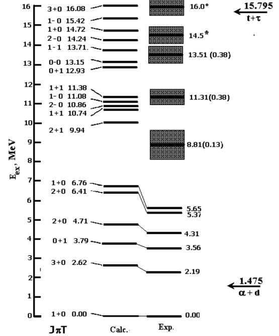
Fig. 5. Schematic diagram of the {}^6\text{Li} nucleus levels
