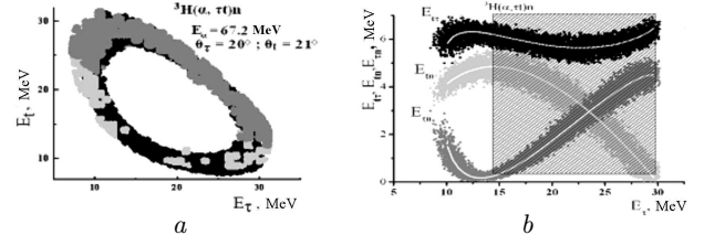
Fig. 7. Upper (gray) and lower (light gray) branches of experimental \tau t -coincidence matrix. The kinematic calculation of the locus position is marked with black background ( a ). Relative energies E_{\tau t} , E_{\tau n} , and E_{tn} of the initial particle pairs in comparison with the energies of \tau -particles calculated in the point geometry framework (solid curves). The results of corresponding Monte Carlo calculations are presented as point arrays. The shaded area corresponds to the energy interval E_{\tau} = (15 \div 31) MeV where the excited {}^6\text{Li} levels are populated and decay into \tau t clusters ( b )
