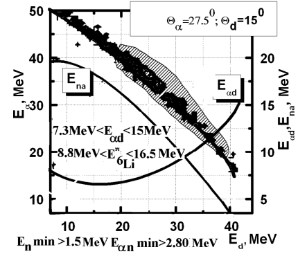
Fig. 3. Two-dimensional \alpha d -coincidence spectrum of the {}^3\text{H}(\alpha, d\alpha)n reaction ( E_\alpha = 67.2 MeV). The shaded area marks the experimental events of resonance formation. Curves E_{n\alpha} and E_{\alpha d} demonstrate the calculated relative energies in the n + \alpha and d + \alpha pairs, respectively
