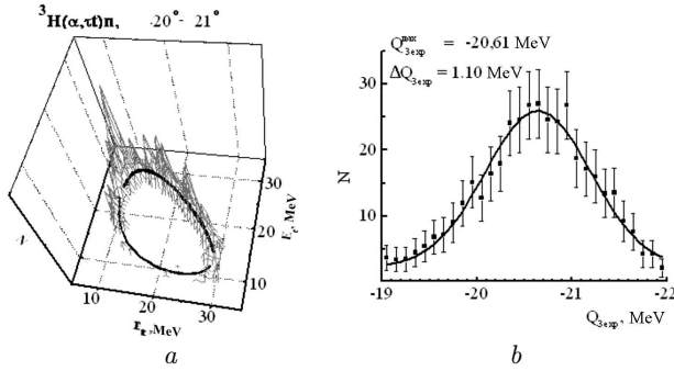
Fig. 6. Two-dimensional experimental \tau t coincidence spectrum; the solid line represents the kinematic curve calculated in the framework of point kinematics for the corresponding experimental conditions (a). The corresponding experimental Q_3 spectrum (b)
