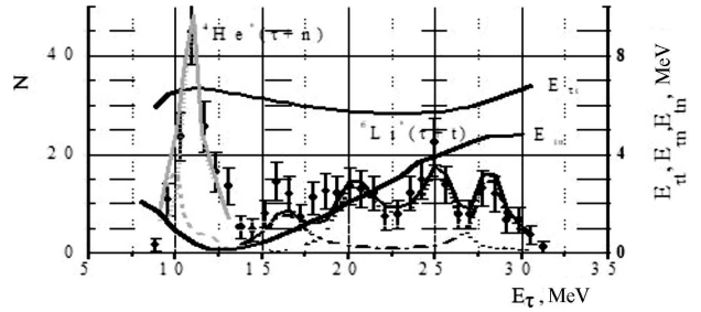
Fig. 8. Projection of the upper branch of two-dimensional \tau - t spectrum obtained at \Theta_t = 21^\circ and \Theta_{\tau} = 20^\circ and an incoming energy of 67.2 MeV of \alpha -particle beam onto the E_{\tau} axis. Curves E_{\tau t} and E_{\tau n} are relative energies in the \tau + t and t + n pairs. The first (light gray) peak is associated with the formation and decay of the second (light gray dashed curve) and third (light gray dotted curve) excited {}^4\text{He} levels. The consecutive dash-double-dotted curve corresponds to the relative energy E_{tn} for the analysis of the contribution made by the excited {}^4\text{H}^* state
