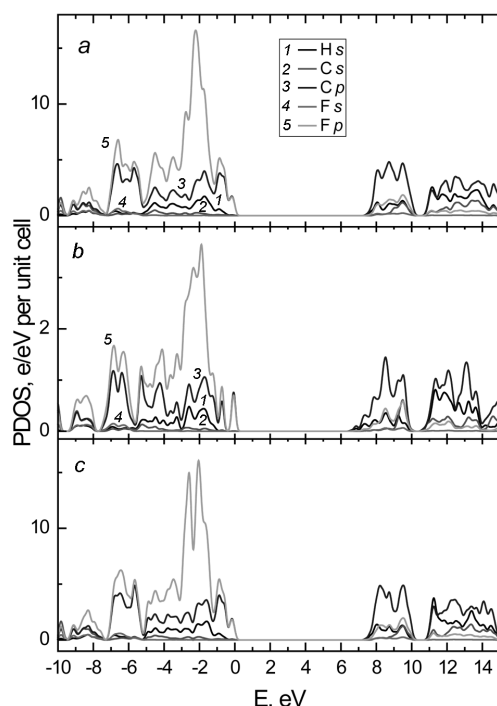
Fig. 4. Calculated partial densities of electronic states of the \alpha - (a), \beta - (b), and \gamma -phase (c) of the PVDF crystal
