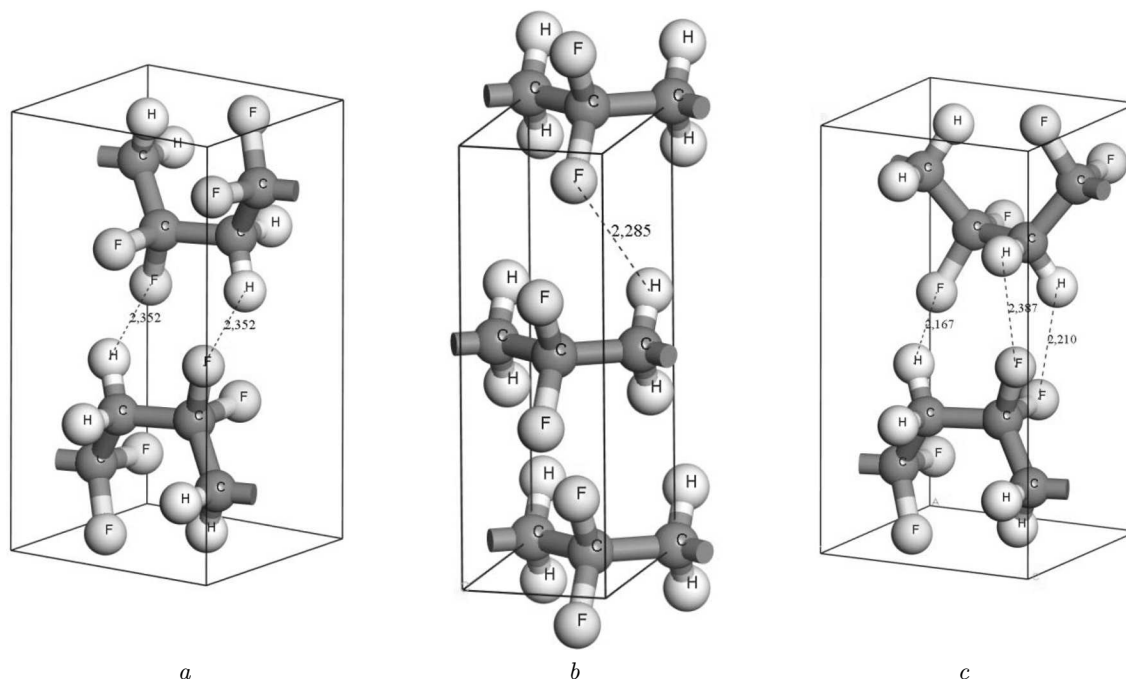
Fig. 1. The structure of the unit cells of \alpha - (a), \beta - (b), and \gamma -phase of a PVDF crystal (c)
