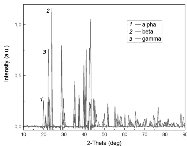
Fig. 2. Calculated angular dependences of the X-ray diffraction intensity (diffractograms) of the \alpha -, \beta -, and \gamma -phase of the PVDF crystal (black (1), red (2), and blue (3) curves, respectively)
