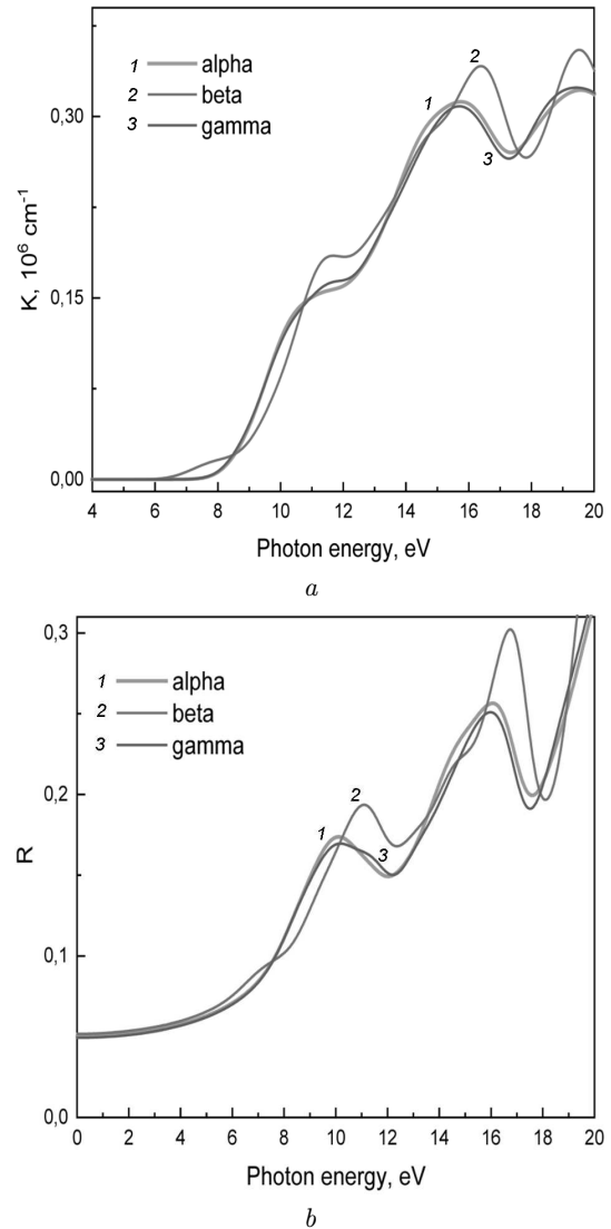
Fig. 7. Calculated absorption (a) and reflection (b) spectra of \alpha -, \beta -, and \gamma -phase PVDF crystals (green (1), red (2), and blue (3) curves, respectively)
