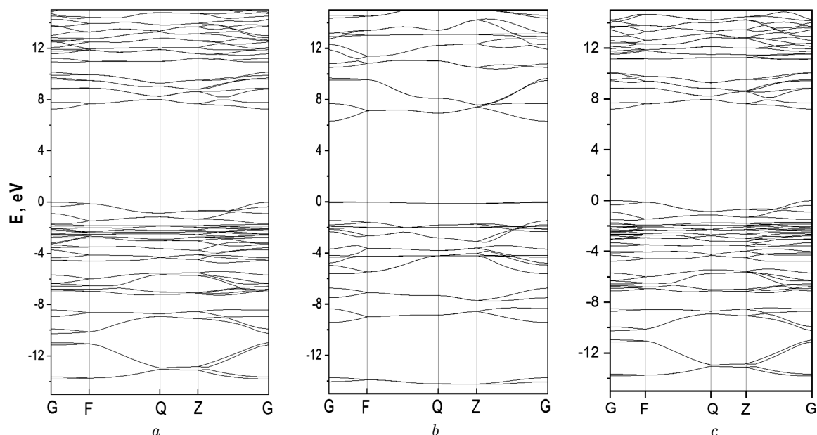
Fig. 3. The calculated band structure of \alpha - (a), \beta - (b), and \gamma -phase PVDF crystals (c)
