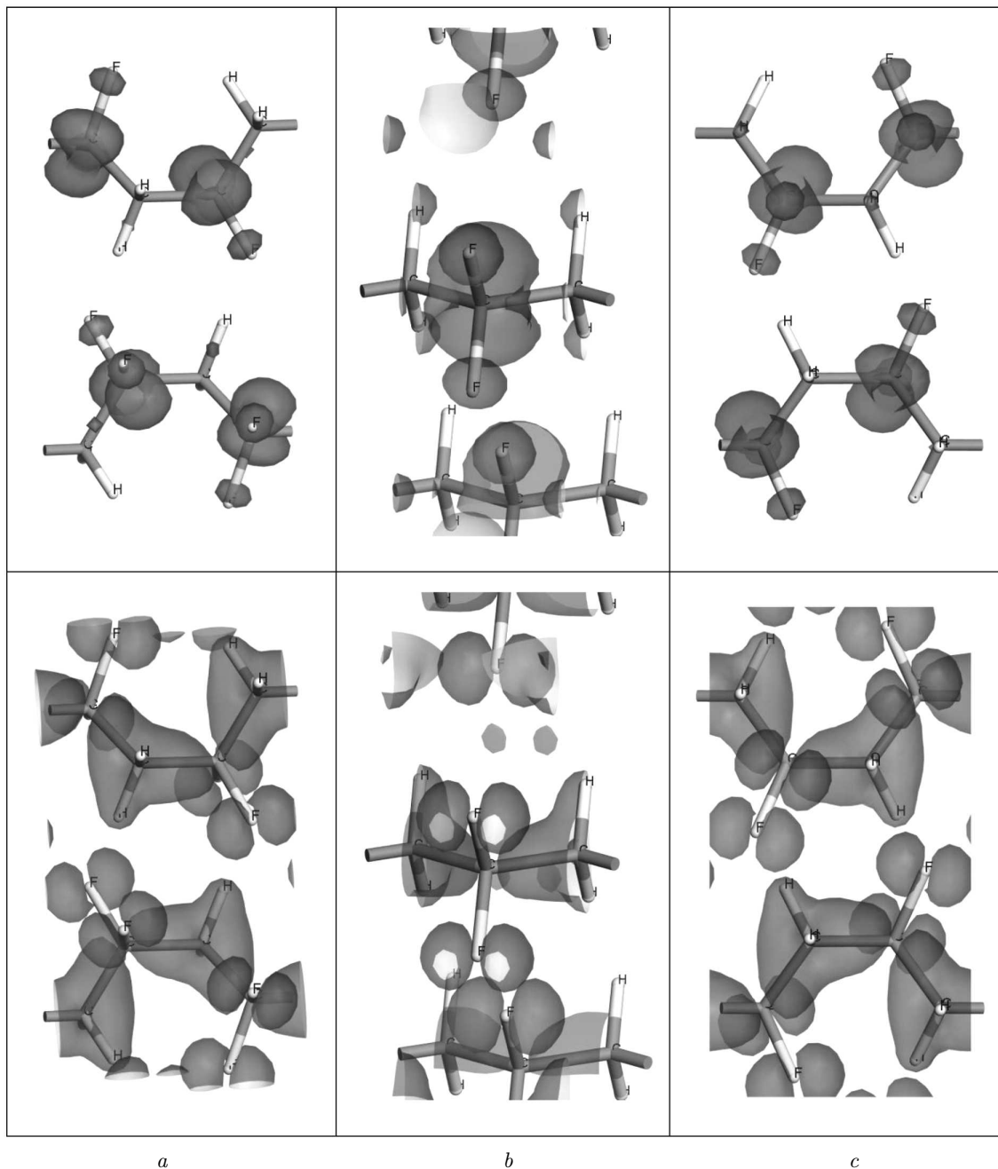
Fig. 5. Calculated spatial distributions of electron density in the energy regions of the top of the Valence band (bottom row) and the bottom of the Conduction band (top row) of \alpha - (a), \beta - (b), and \gamma -phase (c) of a PVDF crystal. The blue isosurfaces correspond to 0.04 e level of electron density
