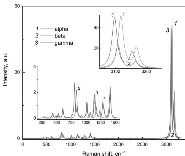
Fig. 8. Calculated Raman spectra of the \alpha -, \beta -, and \gamma -phases of the PVDF crystal (green (1), red (2), and blue (3) curves, respectively). The detailed structure of the spectra is shown in the insets
