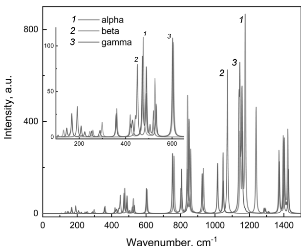
Fig. 9. Calculated infrared absorption spectra of the \alpha -, \beta -, and \gamma -phases of a PVDF crystal (green (1), red (2), and blue (3) curves, respectively). The inset shows the details of the spectra in the long-wave region
