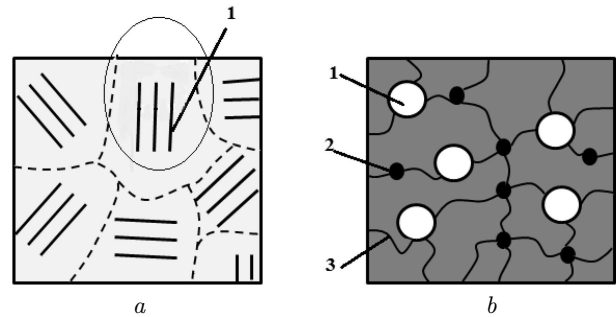
Fig. 4. Schematic diagrams of the gel structure (a) and the local equilibrium region (b): fiber (1), network node (2), and chain (3)
