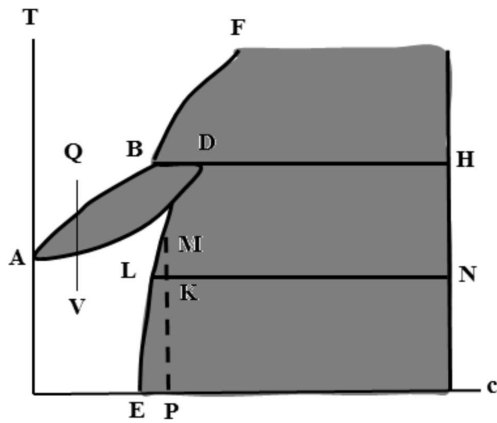
Fig. 3. Phase diagram for the “gelatin–water” system
