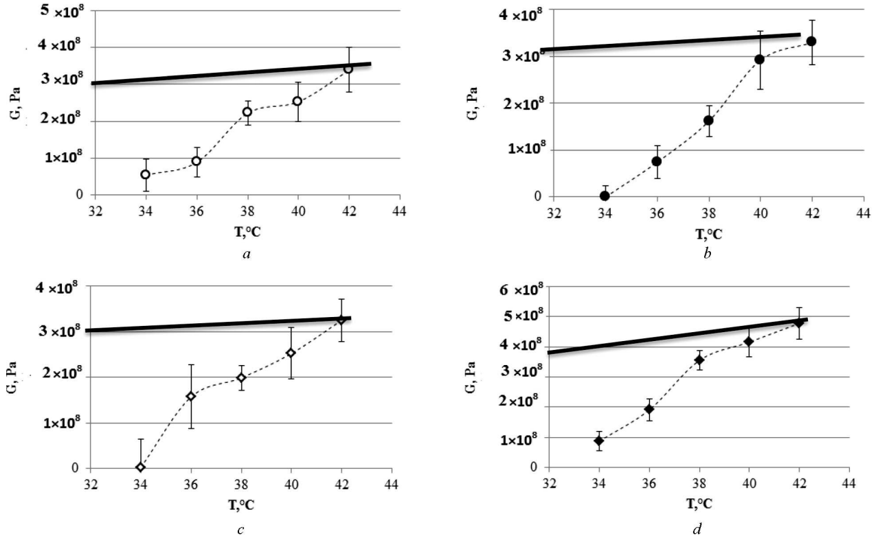
Fig. 2. Temperature dependences of the shear modulus G in gelatin hydrogel with various gelatin concentrations 12% (a), 20% (b), 30% (c), and 40% (d)
