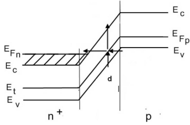
Fig. 2. Energy band diagram of the n^+-p junction at large reverse bias. Direct tunneling transitions from the valence band into the conduction band are possible for charge carriers of group (d)
