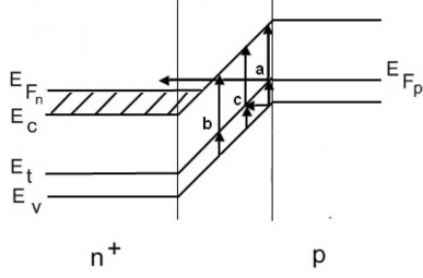
Fig. 1. Energy band diagram of the n^+-p junction at a small reverse bias. Vertical and horizontal arrows show possible thermally induced and tunneling, respectively, transitions for three groups of charge carriers (a, b, and c) [20]
