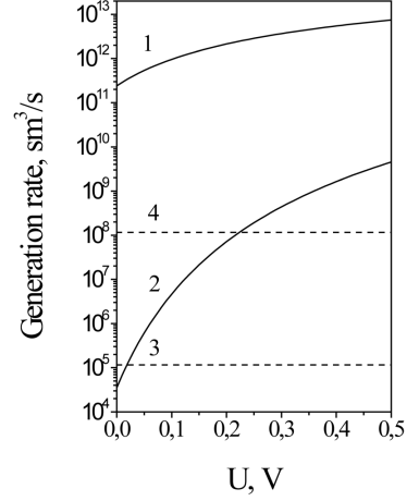
Fig. 3. Tunneling generation rates of holes, \omega_v N_v (1), and electrons, \omega_c N_c (2), for the trap level E_t - E_v = 0.28 E_g . The thermally induced generation rate was calculated for C_p = 10^{-9} (3) and 10^{-6} \text{ cm}^3/\text{s} (4)
