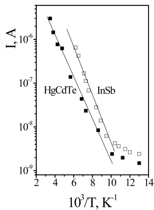
Fig. 7. Arrhenius dependences for the reverse current in the HgCdTe and InSb photodiodes at a bias voltage of 10 mV. Solid lines are drawn for averaged data
