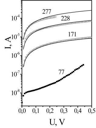
Fig. 8. Reverse CVCs for the HgCdTe photodiode at various temperatures (in kelvins). Solid lines are the results of calculations of generation current when the trap level is in the middle of the bandgap (see explanations in the text)
