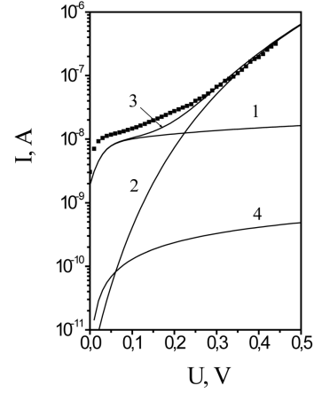
Fig. 9. Reverse CVCs for the HgCdTe photodiode at T = 77 K. Solid curves are the results of calculations of the TAT current according to formulas (9) and (10) for the trap levels in the lower (curve 1) and upper (curve 2) halves of the bandgap, and the total current (curve 3). Curve 4 is the Shockley generation current for the level in the middle of the bandgap
