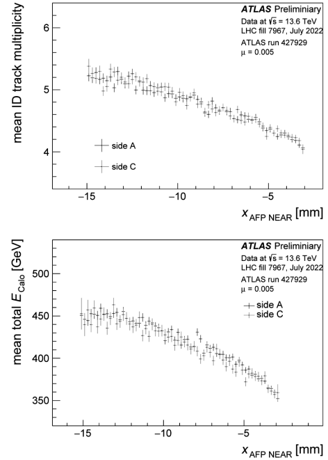
Fig. 17. Correlation of the AFP track x-position to the charged track multiplicity of the ATLAS Inner Detector (ID), and correlation of the AFP track x-position to the total energy measured by ATLAS calorimeters (from [5])
