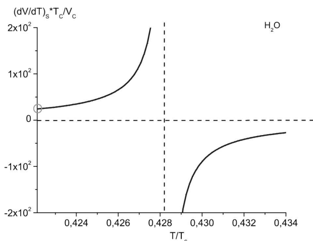
Fig. 2. Temperature dependence of the thermodynamic coefficient (\partial V/\partial T)_S \cdot T_C/V_C along the liquid-vapor coexistence curve for \text{H}_2\text{O} in the temperature interval T < 4^\circ\text{C} . The vertical dashed line marks a characteristic temperature of 4^\circ\text{C} . The triple point is marked with a circle
