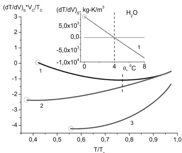
Fig. 3. Temperature dependences of the thermodynamic coefficient (\partial T/\partial V)_S \cdot V_C/T_C along the liquid-vapor coexistence curve for \text{H}_2\text{O} (1), \text{H}_2\text{O}_2 (2), and Ar (3). The vertical dashed line marks a temperature of 223.1^\circ\text{C} (the minimum of (\partial T/\partial V)_S \cdot V_C/T_C for \text{H}_2\text{O} ). The circles mark the triple points for \text{H}_2\text{O} , \text{H}_2\text{O}_2 , and Ar. The temperature dependence of (\partial T/\partial V)_S around 4^\circ\text{C} for \text{H}_2\text{O} is shown in the inset; the vertical dashed line marks a temperature of 4^\circ\text{C}
