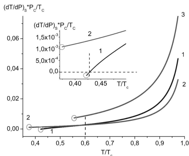
Fig. 4. Temperature dependences of the thermodynamic coefficient (\partial T/\partial P)_S \cdot P_C/T_C along the liquid-vapor coexistence curve for \text{H}_2\text{O} (1), \text{H}_2\text{O}_2 (2), and Ar (3). The vertical dashed line marks a temperature of 102.2^\circ\text{C} (the inflection point of (\partial T/\partial P)_S \cdot P_C/T_C for \text{H}_2\text{O} ). The inset shows the relative temperature interval T/T_C < 0.5 . The vertical dashed line marks a temperature of 4^\circ\text{C} (characteristic of \text{H}_2\text{O} ). The circles mark the triple points for \text{H}_2\text{O} , \text{H}_2\text{O}_2 , and Ar
