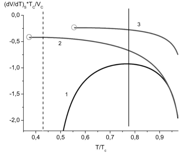
Fig. 1. Temperature dependences of the thermodynamic coefficient (\partial V / \partial T)_S \cdot T_C / V_C along the liquid-vapor coexistence curve for H 2 O (1), H 2 O 2 (2), and Ar (3). The vertical dashed line marks a temperature of 4 °C characteristic of water. The vertical solid line marks a temperature of 223.1 °C (the maximum of the quantity (\partial V / \partial T)_S \cdot T_C / V_C for H 2 O). The circles mark triple points for H 2 O 2 and Ar
