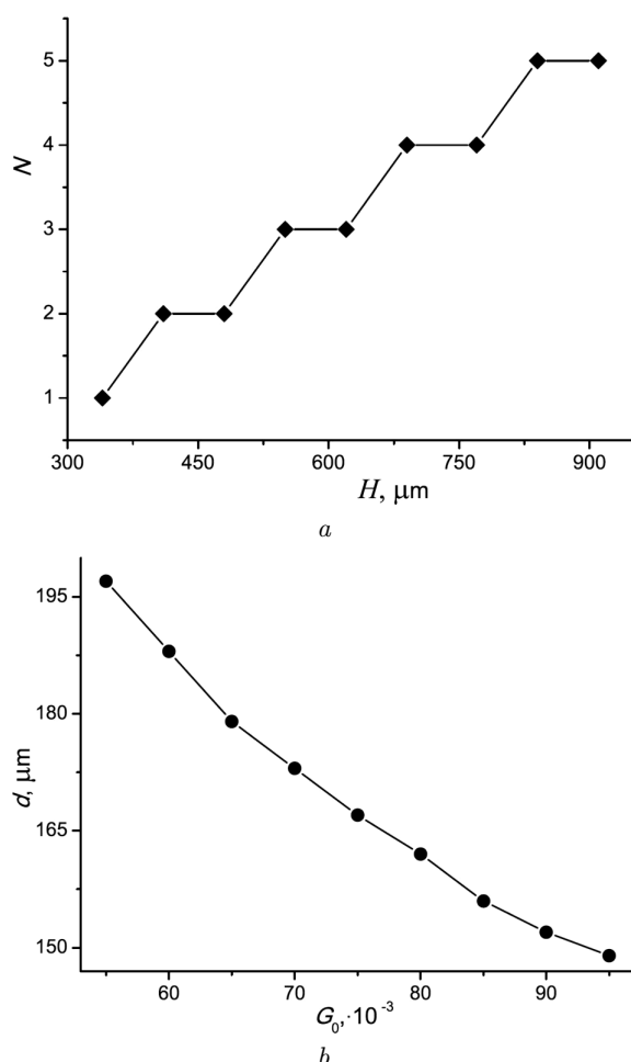
Fig. 6. Dependence of the number of EHL island rows in the stripe on the stripe thickness at fixed uniform stripe pumping (a); dependence of the distance between islands in a row on the pumping intensity (b)
