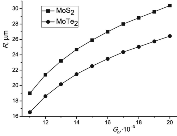
Fig. 2. Critical radius of EHL island
