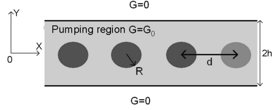
Fig. 3. Formation of EHL droplets from the exciton gas in the case of uniform irradiation of TMD in the narrow-stripe pumping mode
