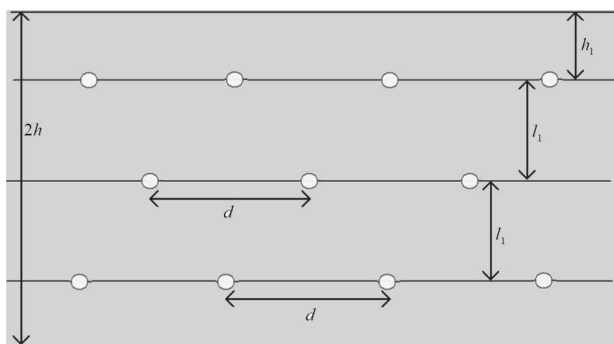
Fig. 5. Optimal arrangement of EHL islands in the case of uniform irradiation of TMD in the wide-stripe pumping mode
