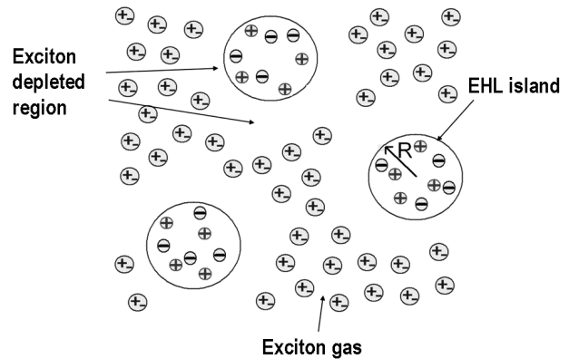
Fig. 1. Schematic diagram for the formation of EHL islands from the exciton gas
