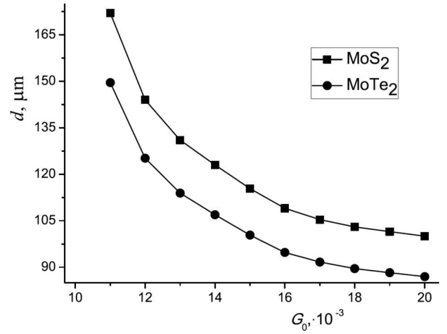
Fig. 4. Distance between EHL islands in a dichalcogenide monolayer in the case of uniform irradiation of TMD in the narrow-stripe pumping mode
