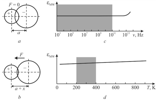
Fig. 2. Ionic polarization: simplest model consisting of one positive and one negative ion (a); deformation x in local field F (b); frequency dependence of the ionic permittivity (c); ionic permittivity temperature dependence (shaded areas show the range of technical interest) (d)
