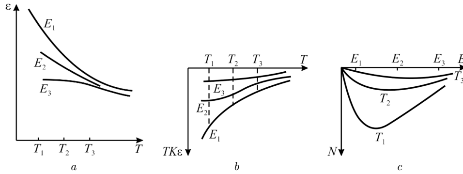
Fig. 7. Nonlinearity of permittivity in paraelectrics: permittivity dependence on temperature and bias field (a); temperature dependence TC\epsilon (b); non-linearity dependence on temperature and bias field (c)
