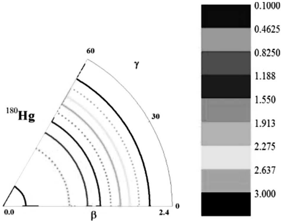
Fig. 3. The PES contour plot for ^{180}\text{Hg} nucleus
