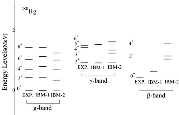
Fig. 2. The level scheme of different type of bands: ground (a), gamma (b) and beta (c) in ^{180}\text{Hg} nucleus are mutually compared with presented by IBM-1 and IBM-2 models and previously measured data
