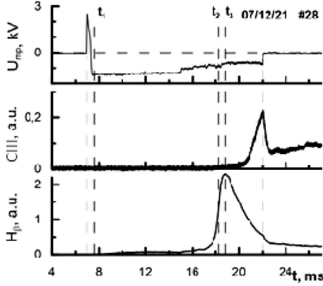
Fig. 8. The same as in Fig. 6, but for P = 1.7 \times 10^{-4} Torr
