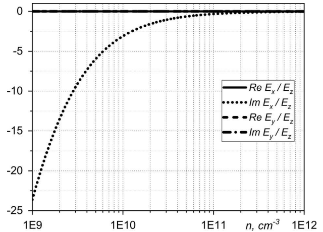
Fig. 13. Dependences of the amplitude ratios between the electric field components of the slow wave on the plasma concentration for B = B_0 and l = 10
