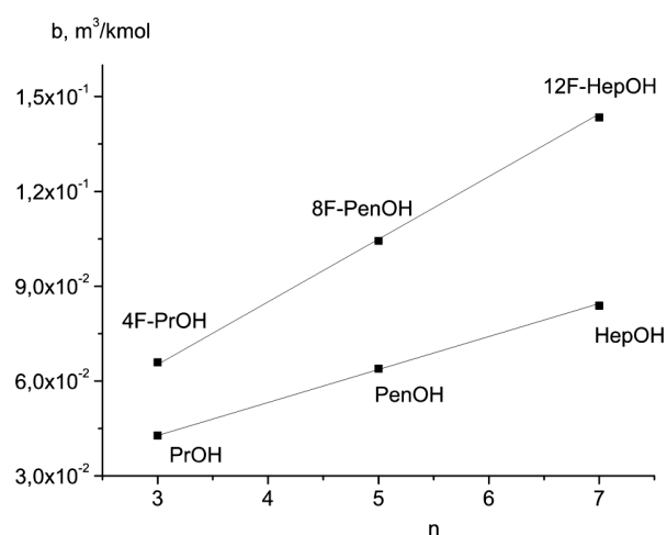
Fig. 9. Dependences of the intermolecular Van der Waals interaction parameter b on the number of carbon atoms n in the molecule for aliphatic alcohols and their fluoro-substituted analogs
