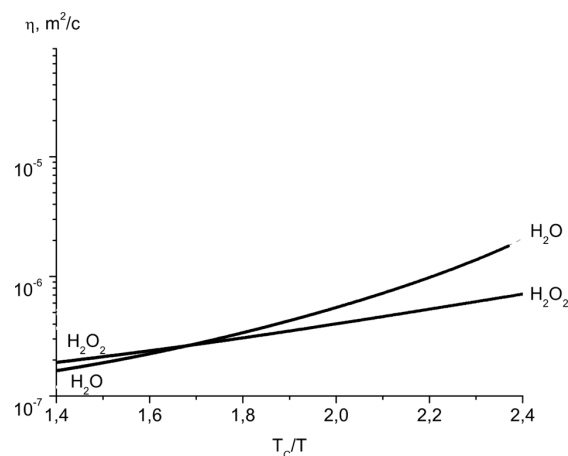
Fig. 5. Temperature dependences of the logarithm of shear viscosity for water and hydrogen peroxide
