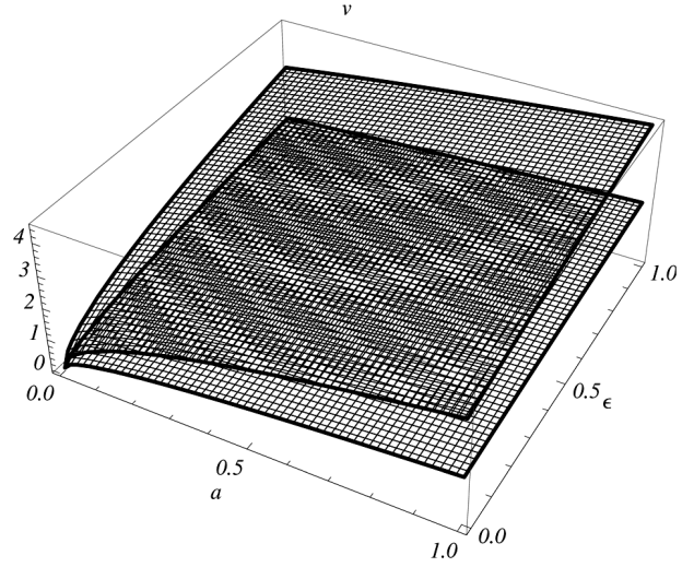
Fig. 3. The velocity v as a function of the scale factor a and the parameter \varepsilon = \frac{E}{2M} for different values of M and Q = 0 . See the caption to Fig. 2
