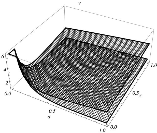
Fig. 2. The velocity v as a function on the scale factor a and the parameter \epsilon = \frac{E}{2M} . The lower surface corresponds to the value 2M = 2 , and the upper surface to 2M = 10
