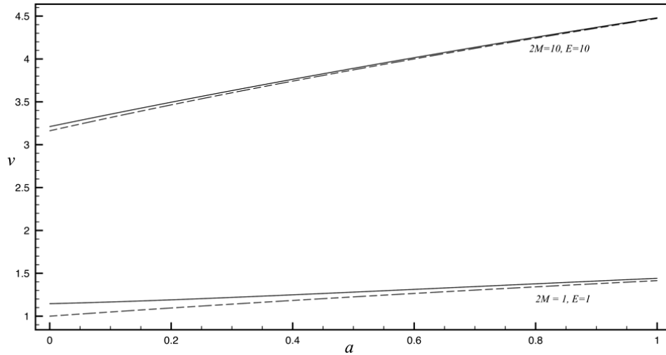
Fig. 1. The velocity v as a function on the scale factor a for different values of the parameters M and E . Dotted lines correspond to the cases Q = 0
