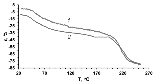
Fig. 3. Thermomechanical analysis results of samples A (1) and B (2)
