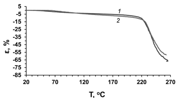
Fig. 7. Results of thermomechanical analysis of samples C (1) and D (2)
