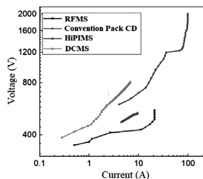
Fig. 3. Current-voltage curves of the standard and linear triple magnetron sputtering methods [13]
