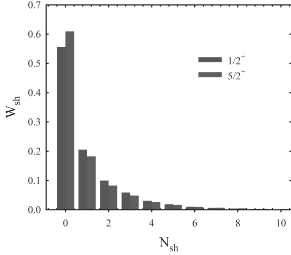
Fig. 3. Weights of different oscillator shells to the wave functions of 1/2^+ and 5/2^+ states in {}^7\text{Li}
