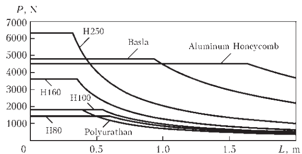
Figure 4. Critical load versus span length for failure initiation in sandwich beams under three-point bending. Horizontal lines indicate core shear failure and curved lines indicate failure by compressive facing wrinkling
