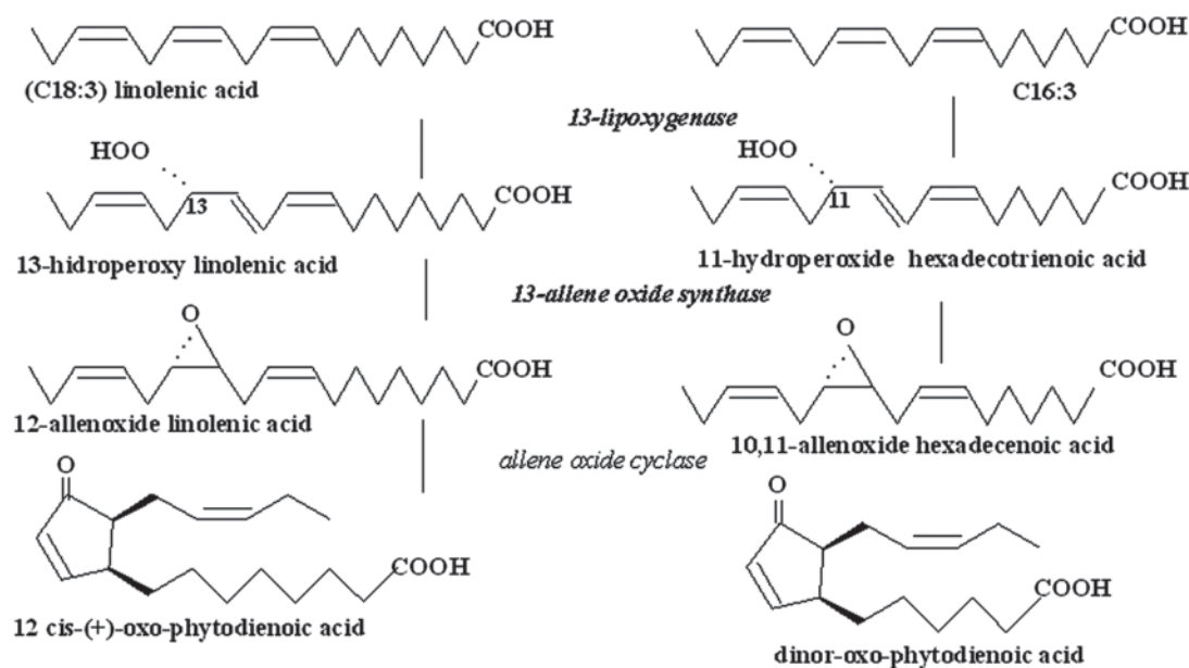
Fig. 1. Schematic diagram of the jasmonic acid synthesis first stage that begins in chloroplasts (cited data by Wasternack, Forner, 2013)
