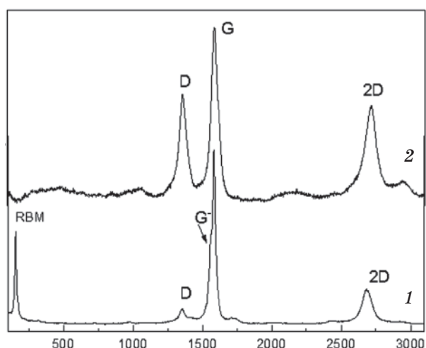
Fig. 3. Raman spectrum of untreated (1) and functionalized using DNA (2) SWCNTs
