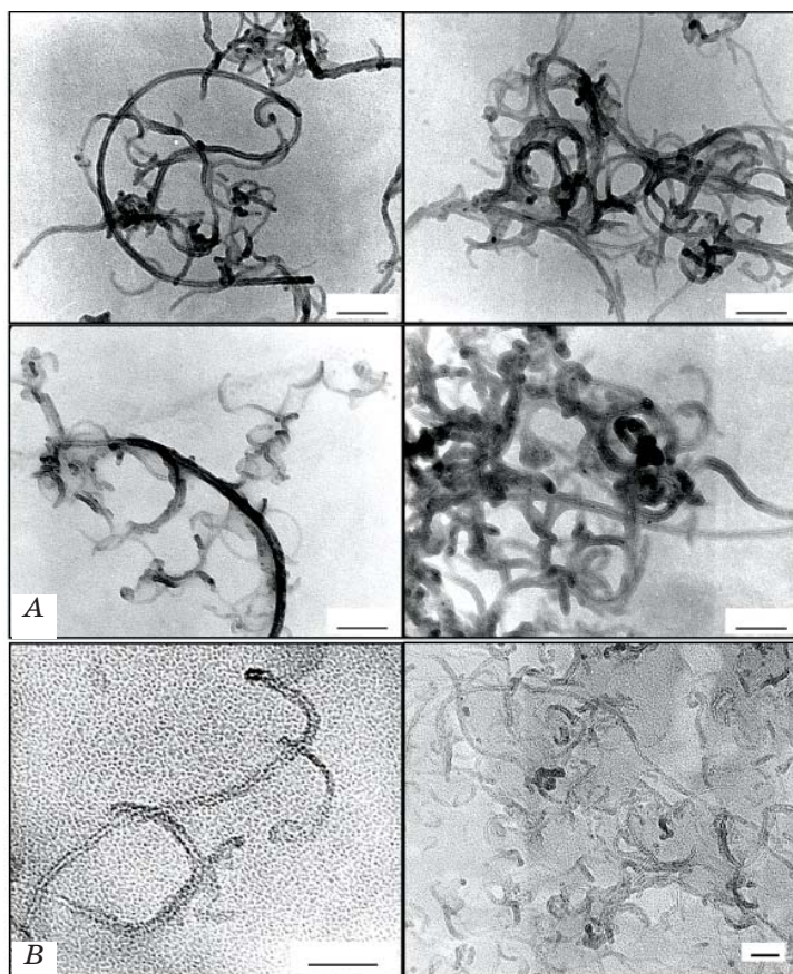
Fig. 2. Transmission electron microscopy image of MWCNTs:
