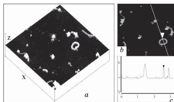
Fig. 4. The results of atomic force microscopy study of samples of MWCNTs functionalized using DNA:
