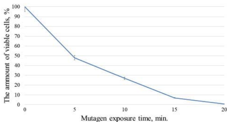
Fig. 1. Cell survival of Brevibacterium sp. IMV B-7447 under the NTG influence at a concentration of 100 \text{ } \mu\text{g/dm}^3
