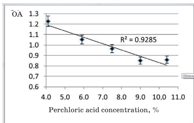
Fig. 3. The influence of different concentrations of \text{HClO}_4 on the chromogenic product yield in the ninhydrin reaction
