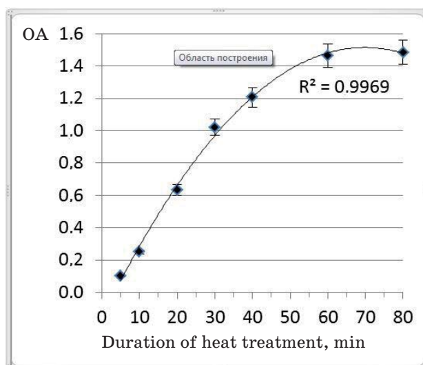
Fig. 4. Quantity dependence of the obtained colored product (optical absorption, 515 \text{ nm} ) on the duration of treatment in a boiling water bath (min)
