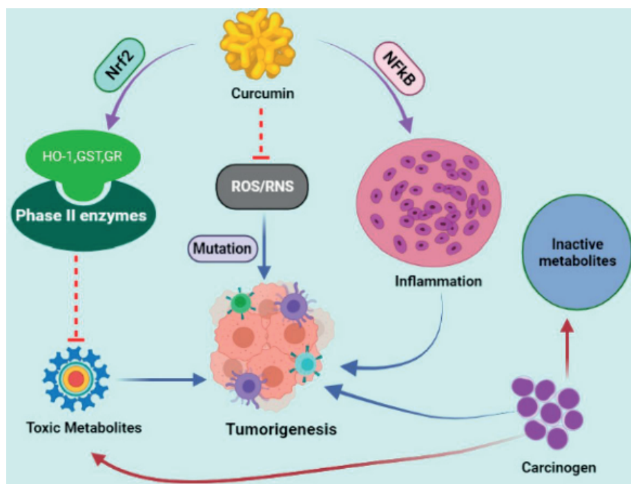
Fig. 3. Effect of curcumin via targeting different pathways including inhibition of ROS (reactive oxygen species); RNS (reactive nitrogen species); NFκB (nuclear factor kappa B); Nrf2 (NF-E2-related factor 2); HO-1(heme oxygenase-1); GST (glutathione S-transferase); GR (glutathione reductase) [71] https://doi.org/10.3390/molecules27010167
