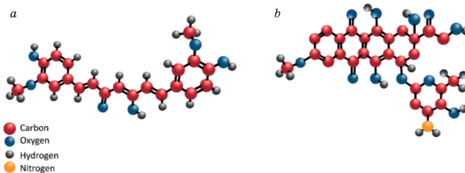
Fig. 2. The chemical structure of curcumin (a) and doxorubicin (b) [27] https://doi.org/10.3390/pharmaceutics12111084
