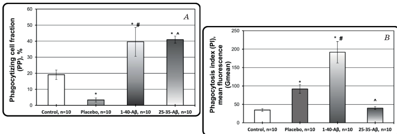
Fig. 1. Phagocytic activity of microglial cells in rats with AD induced by injections of Aβ 1-40 and Aβ 25-35. Phagocytizing cell fraction, PP (A) and phagocytosis index, PI (B). Data are presented as Mean ± SD. Statistical differences are calculated using ANOVA with Tukey's post-hoc test. * and # indicate significant ( P < 0.05 ) differences as compared to the values in intact and sham-operated animals correspondingly, ^ — P \leq 0.05 compared with the rats with AD induced by injections of Aβ1-40.
