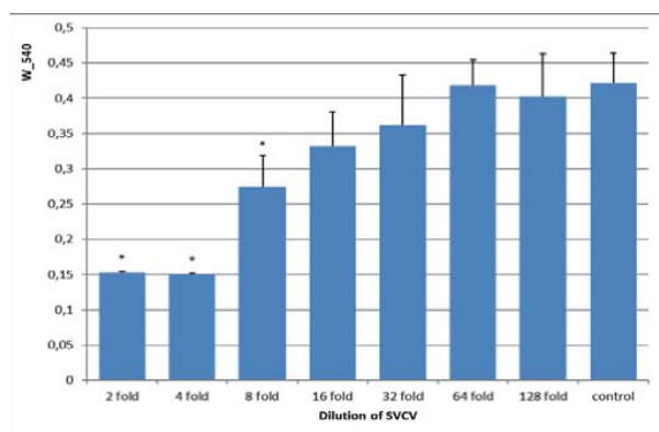
Fig. 1. Effect of SVCV (isolate Svirneve VN17) on cultured HeLa cells (human cervical cancer) at different dilutions. MTT assay data
