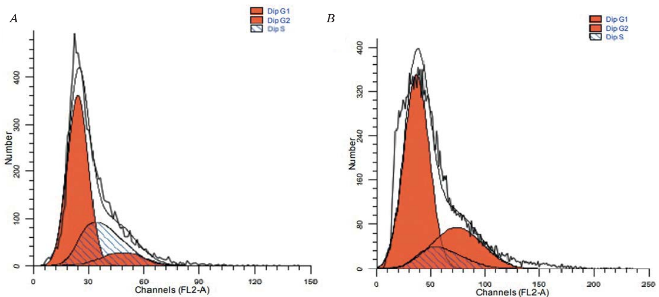
Fig. 3. The cell cycle distribution of HeLa cells treated with SVCV(isolate Svirneve VN17): A — HeLa cells without treatment; B — HeLa cells treated with SVCV at 1:8 dilution (incubation for 2 days in standard CO 2 incubator conditions at 37 °C 100% humidity in RPMI-1640 medium 10% FBS)
