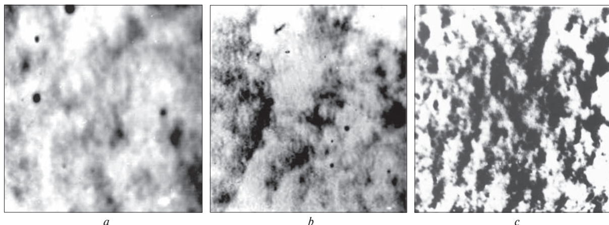
Fig. 3. Examples of different states of the marine environment on the deep horizons: isotherm or weakly stratified (a), stratified (b), thermocline (c)
