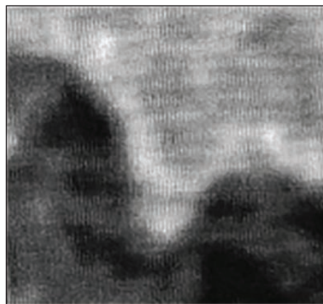
Fig. 1. Fragment of the satellite image of the optical anomaly over the "Schmidt" field
