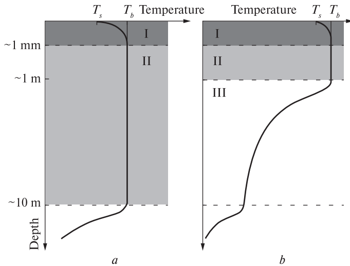
Fig. 2. Idealized temperature profile for night time in winter during strong wind (a) and for daytime in summer during a weak wind (b): I – skin-layer, II – upper bound of the semi homogeneous layer, III – daytime thermocline; T_s – temperature of the skin-layer, T_b – temperature of the upper bound of the semihomogeneous layer
