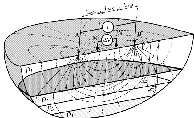
Fig. 1. The principle of conducting VES
