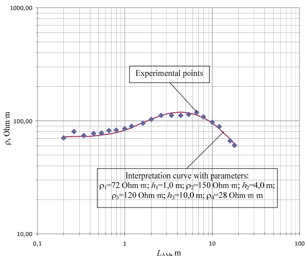
Fig. 3. Interpretation of VES results obtained by the Schlumberger method
