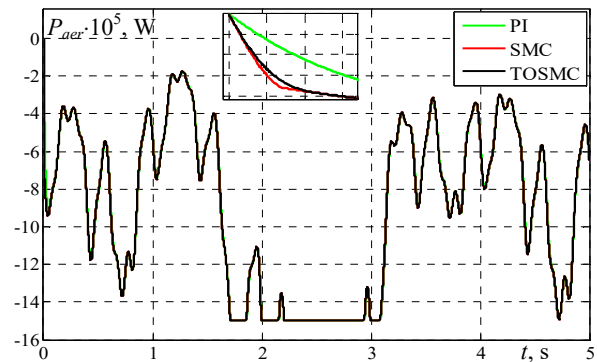
Fig. 6. Aerodynamic power
