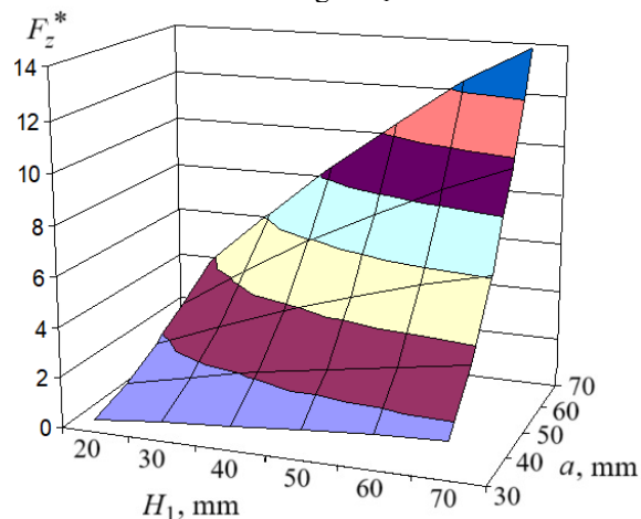
Fig. 6. Dependence of the relative values of the force of attraction of the SMF to the FO on the geometric parameters of the PM
