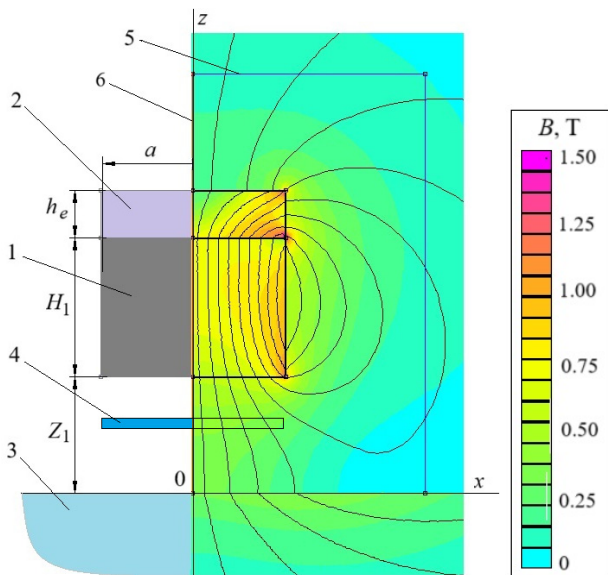
Fig. 2. Schematic diagram of an autonomous SMF as part of a portable EMAT (to the left of the Oz axis) and the distribution of the magnetic field it creates (to the right of the Oz axis): 1 – PM; 2 – FS; 3 – FO; 4 – inductance coil; 5 – calculation limit B_{ex} ; 6 – central axis of the magnetic system
