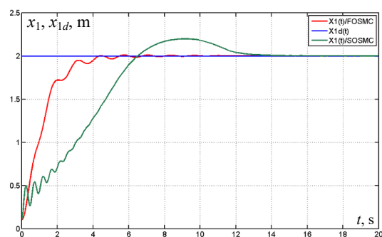
Fig. 9. The output x_1(t) for case 2
