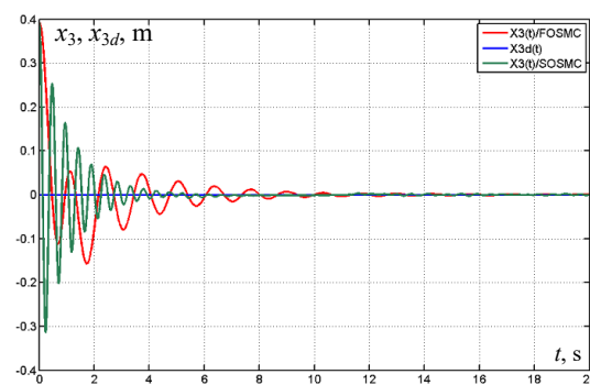
Fig. 10. The output x_3(t) for case 2
