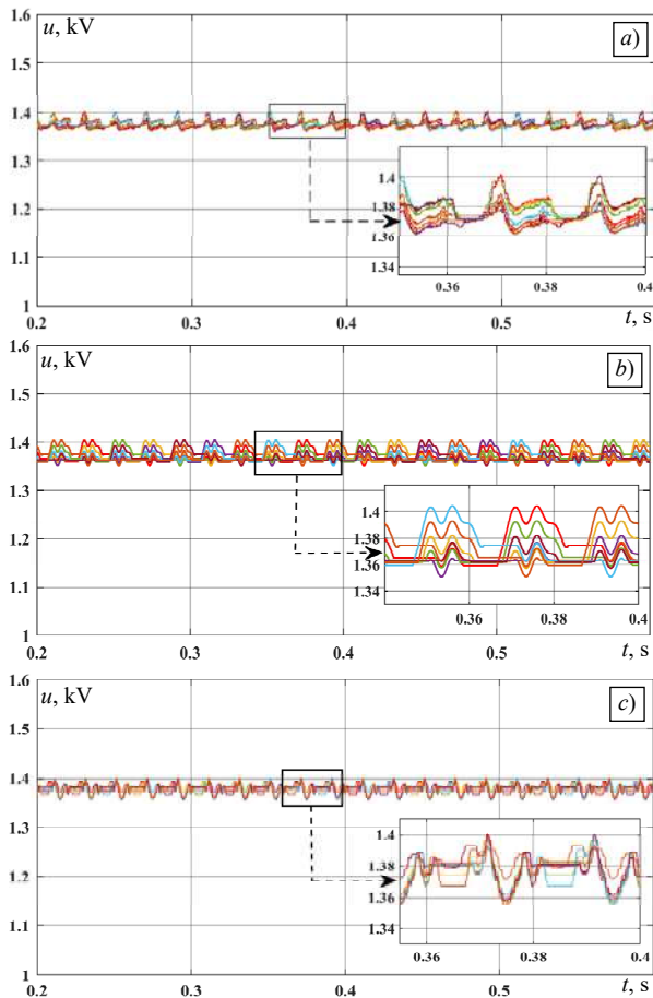
Fig. 14. Capacitor voltages in the upper arm of phase A: LS-PWM (a); NLC (b); NL-PWM (c)
