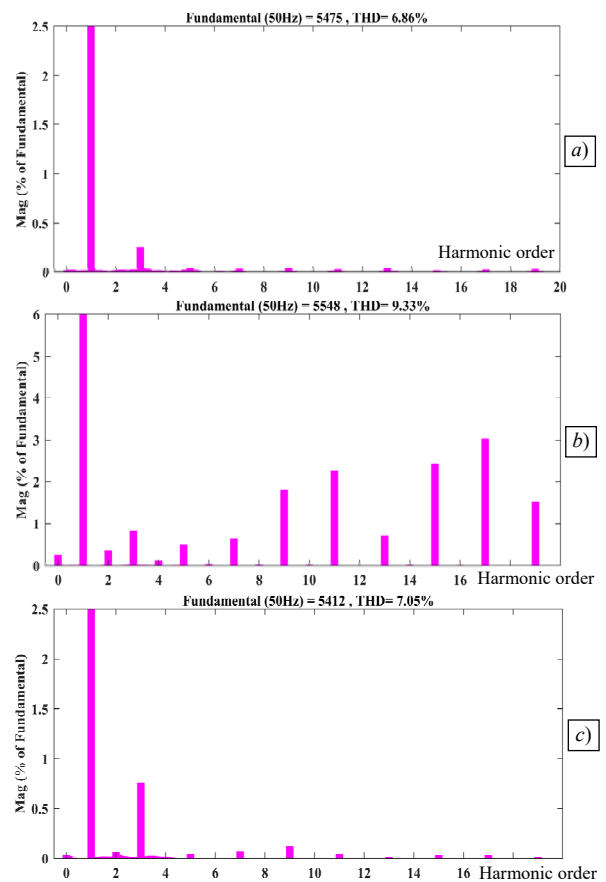
Fig. 13. THD analysis of output voltages: LS-PWM (a); NLC (b); NL-PWM (c)
