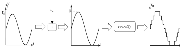
Fig. 5. Principle of the NLC technique
