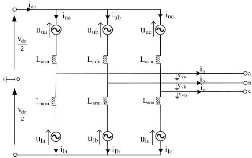
Fig. 3. Equivalent circuit of the MMC
