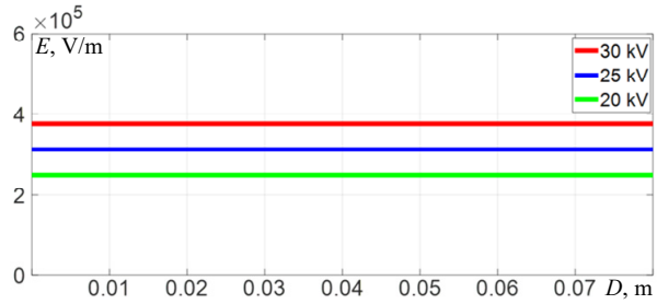
Fig. 8. Electric field variation at the ground for different applied voltages
