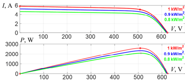
Fig. 4. I - V and P - V characteristics of 14 modules of type ET-M572185 at 25 °C
