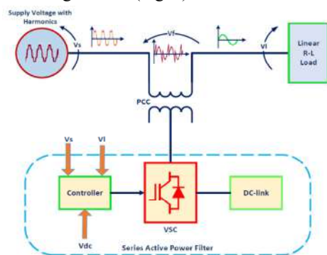
Fig. 2. Modern SAPF
