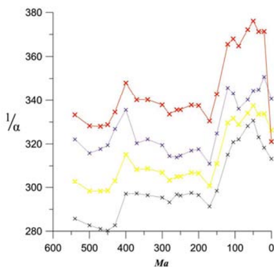
Fig. 9. Changes in compression of a biaxial and triaxial ellipsoids during geological time
