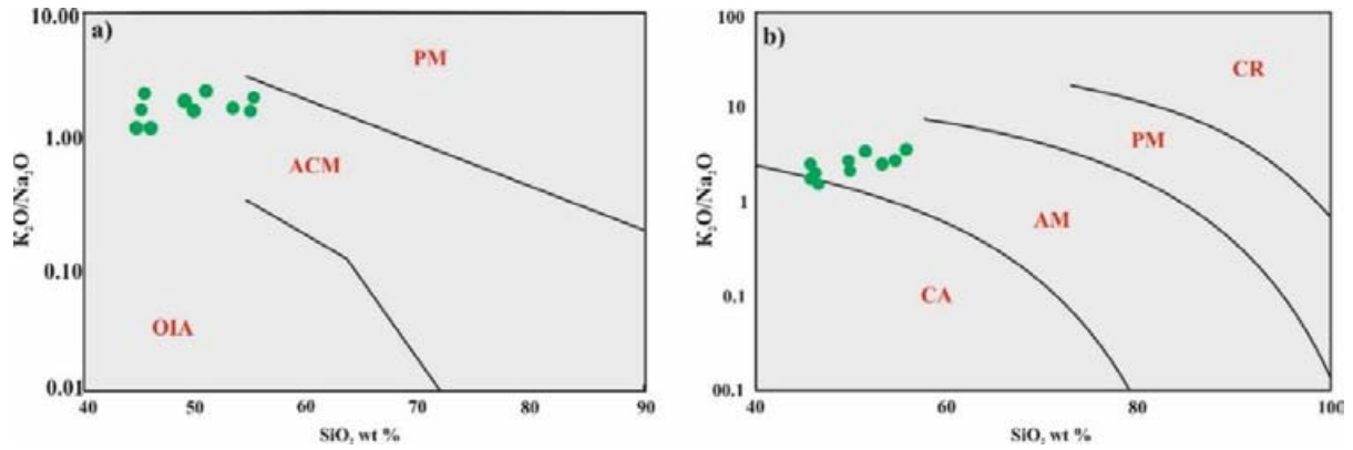
Fig. 13. Tectonic discriminant diagrams are based on the interaction between the SiO 2 value and the K 2 O/Na 2 O ratio for oil shale: a) PM – passive margin, ACM – active continental margin, OIA – oceanic island arc (Roser and Korsch, 1986); b) CR – continental rift, PM – passive margin, AM – active margin, CA – continental arc (Murphy, 2000)
