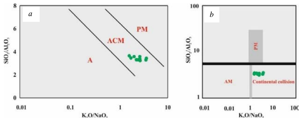
Fig. 12. Tectonic discriminant diagrams based on \text{K}_2\text{O}/\text{Na}_2\text{O} and \text{SiO}_2/\text{Al}_2\text{O}_3 ratios for oil shale samples: a – PM – continental margin, ACM – active continental margin, A – arc (Maynard et al., 1982); b – PM – continental margin, AM – active continental margin (Campos Neto et al. 2011)
