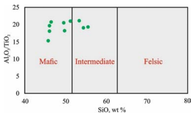
Fig. 7. Association of samples with mafic and intermediate magmatic rocks: the result of SiO 2 versus Al 2 O 3 /TiO 2 diagram (Le Bas et al., 1986)
