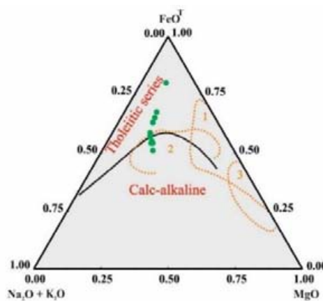
Fig. 9. SiO 2 versus K 2 O diagram (Gill, 1981) (a) and (Na 2 O + K 2 O) – FeO (total) – MgO ternary diagram (Irvine and Bragar) (b) for the samples: fields for (1) island arc non-cumulates, and (2) island arc cumulates after Beard (1986) and (3) ophiolites/cumulates after Coleman (1977) are shown for comparison
